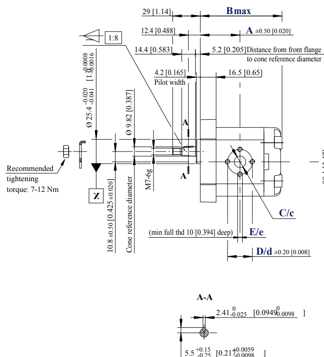
SNP1NN – 01BA and 01DA dimensions
