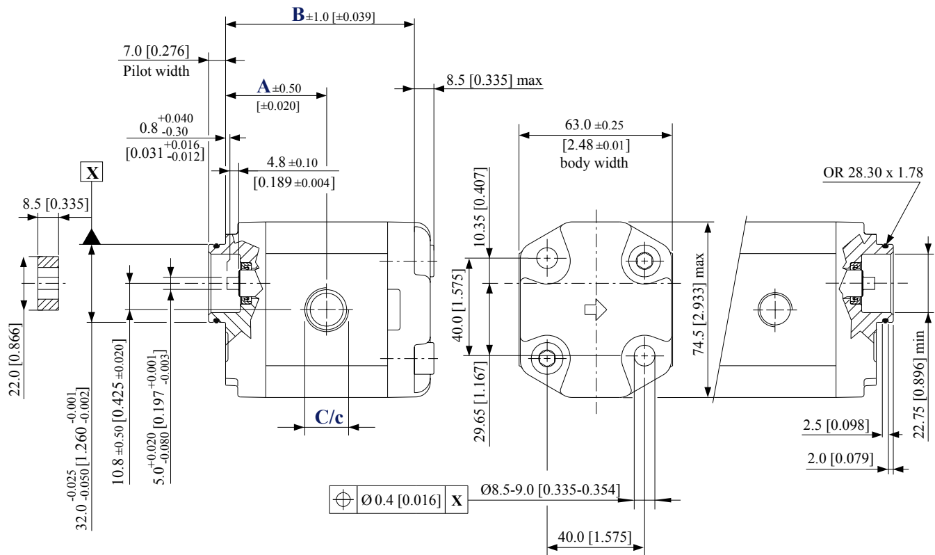
SNP1NN – 03CA dimensions
