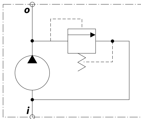
Valve schematic
